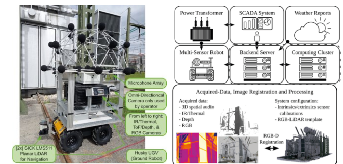
X-AMINOR, 2021–2024 APG, Siemens Energy, Siemens AG, JR DIGITAL Autonomous Multisensoric Transformer Monitoring
